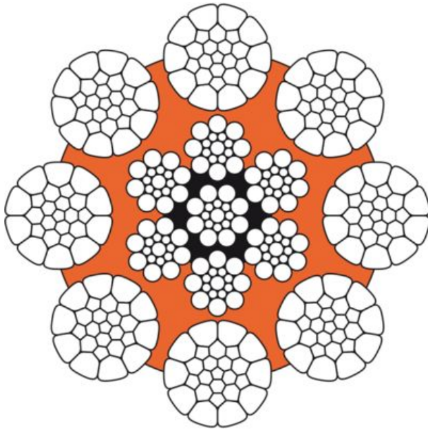
Overhead crane
