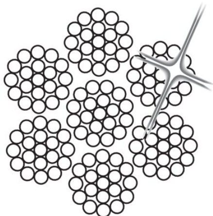
Winch rope
