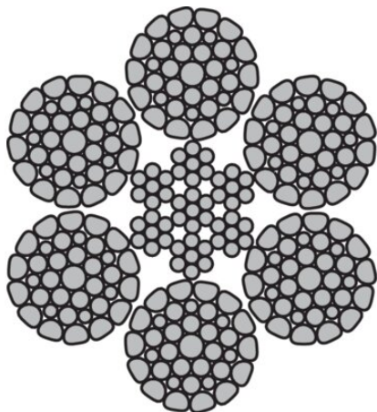
Winch rope
