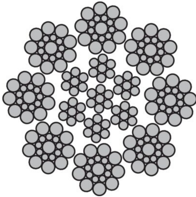
Winch rope
